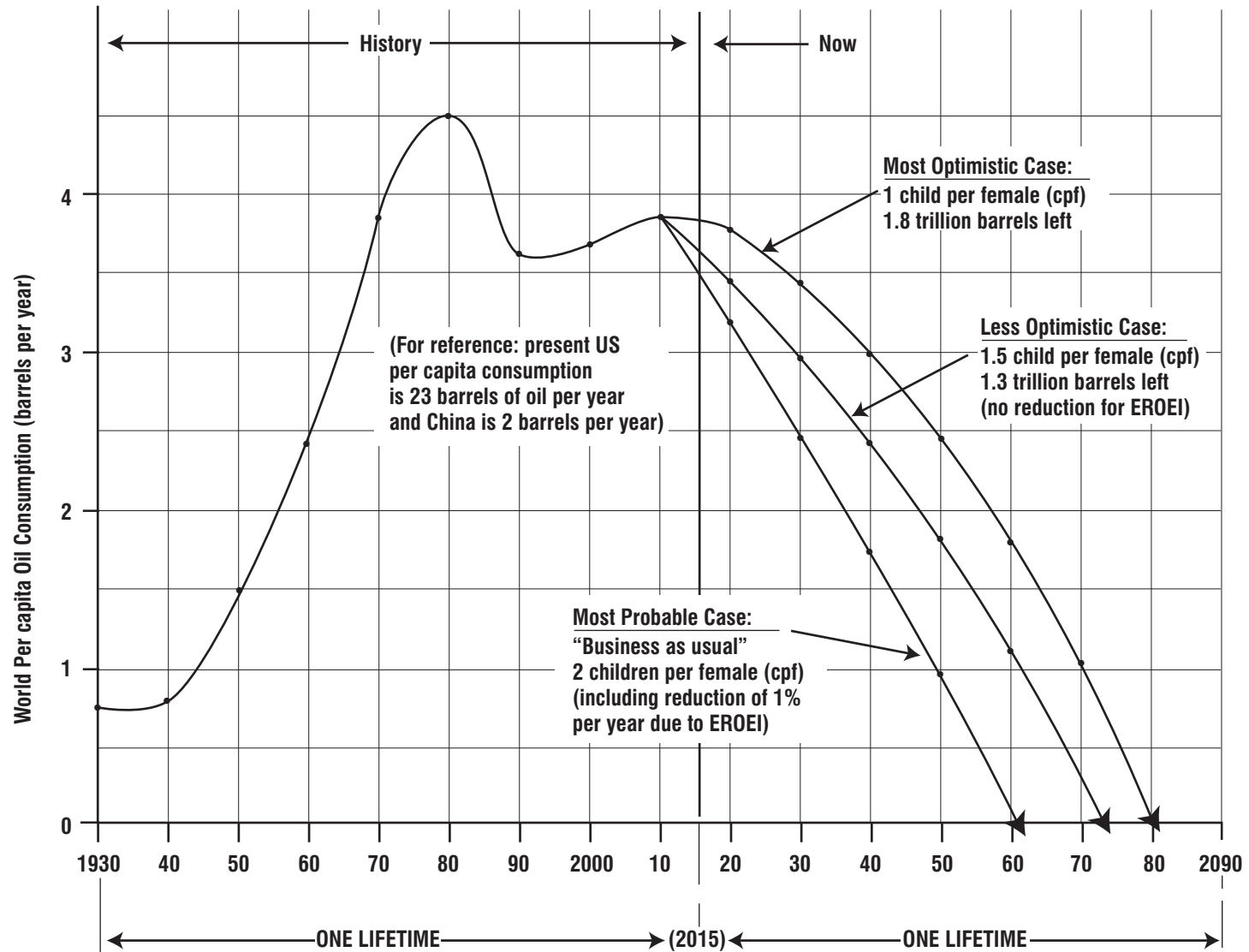
FIGURE 8 Per capita world oil consumption in a two lifetime span
